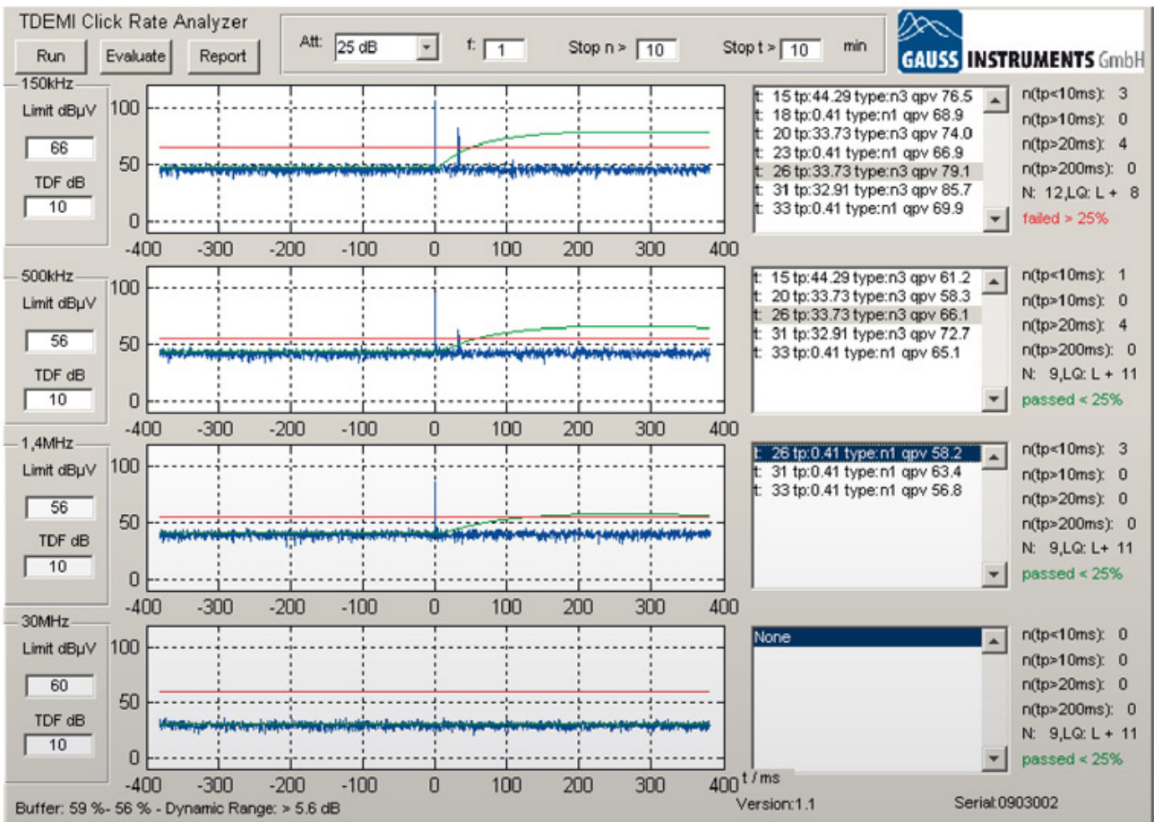
Fig. 1 – Click Rate Analyzer according to CISPR 14 & CISPR 16-2-1
