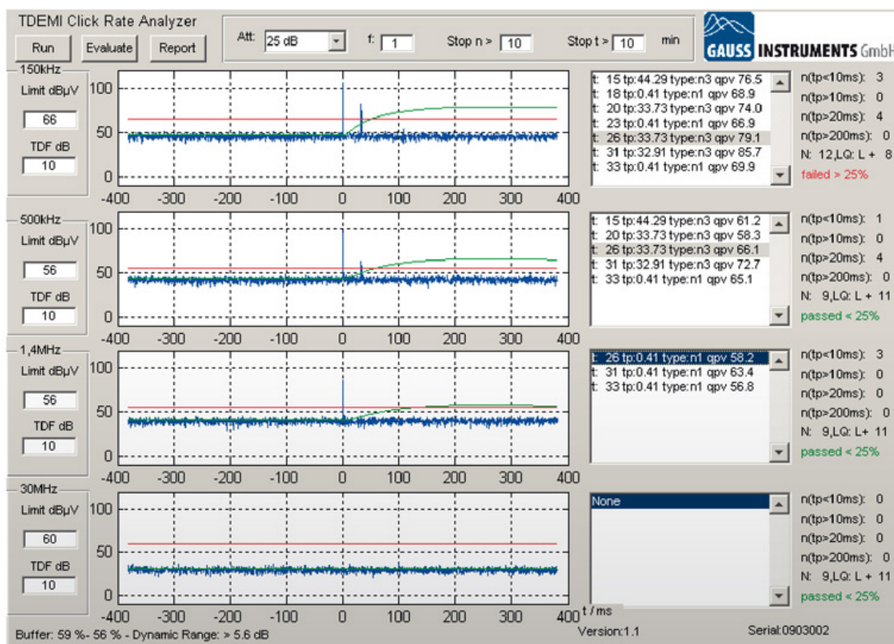
Fig. 1 – Click Rate Analyzer according to CISPR 14 & CISPR 16-2-1
